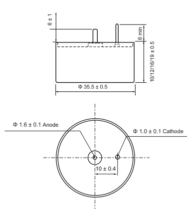
Mounting Dimensional Diagram of HTHC2 Φ35.5 x 10/12/16/19 (Type A)
