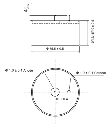
Mounting Dimensional Diagram of HTHC2 Φ35.5 x 10/12/16/19 (Type B)
