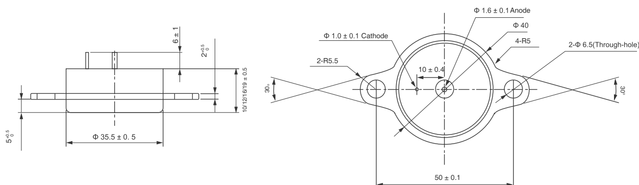
Mounting Dimensional Diagram of HTHC2FB Φ35.5 x 10/12/16/19
